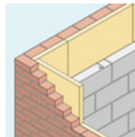
Figure 5. Batts close butted at corners
