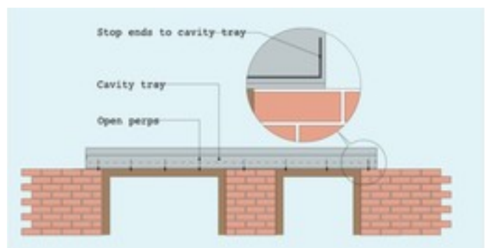
Figure 1. Cavity trays
